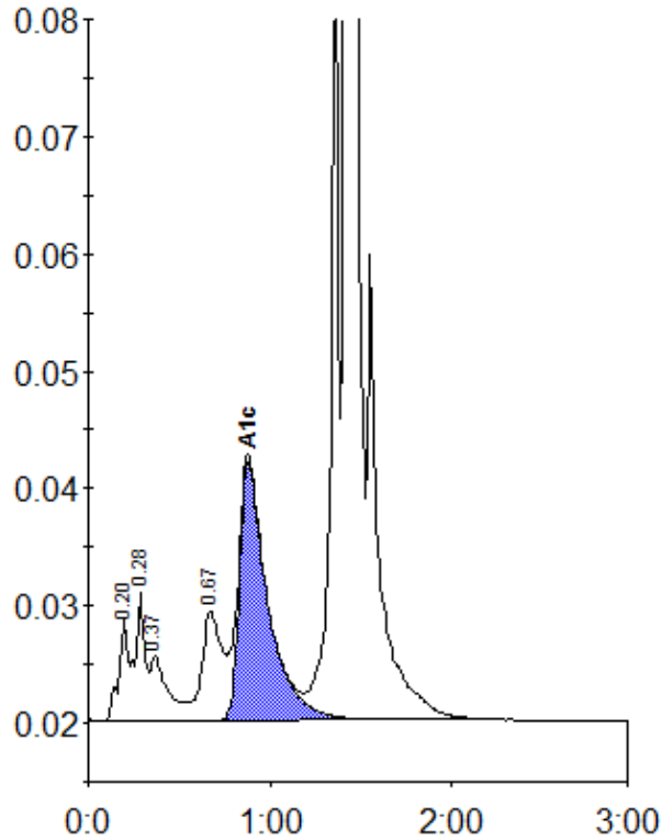
Peak table - ID: 10648447
